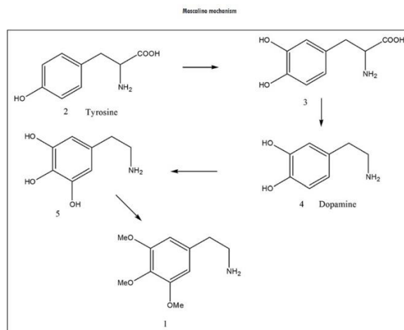
Scheme 1. Biosynthesis of mescaline. Steps include oxidation of (2) to (3), decarboxylation to (4), oxidation to (5) and methylation to (1).
